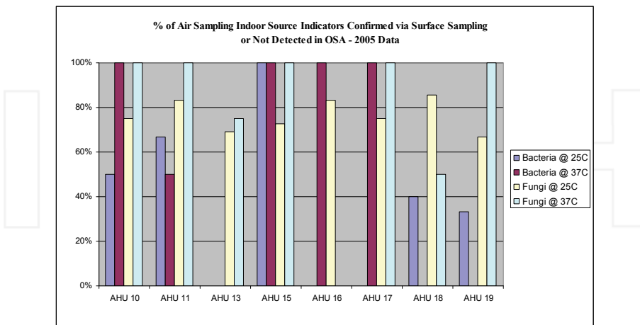
Fig. 7. Percentage of air sampling indoor source indicators confirmed via surface sampling or not detected in the OSA.
